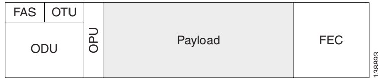
Figure 13 OTN Optical Channel Structure
