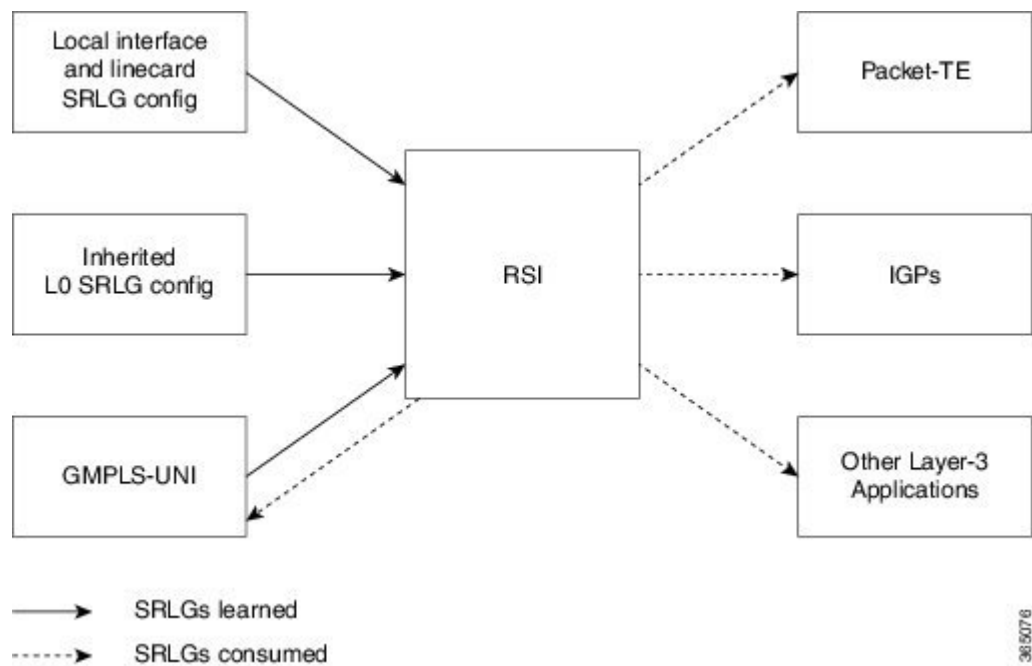
Figure 1: SRLG Communication
