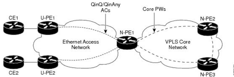
Figure 12: Ethernet Access for H-VPLS
