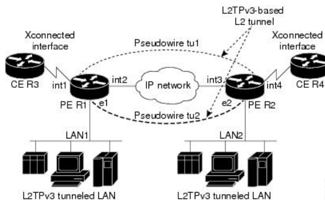
Figure 25: L2TPv3 Operation
