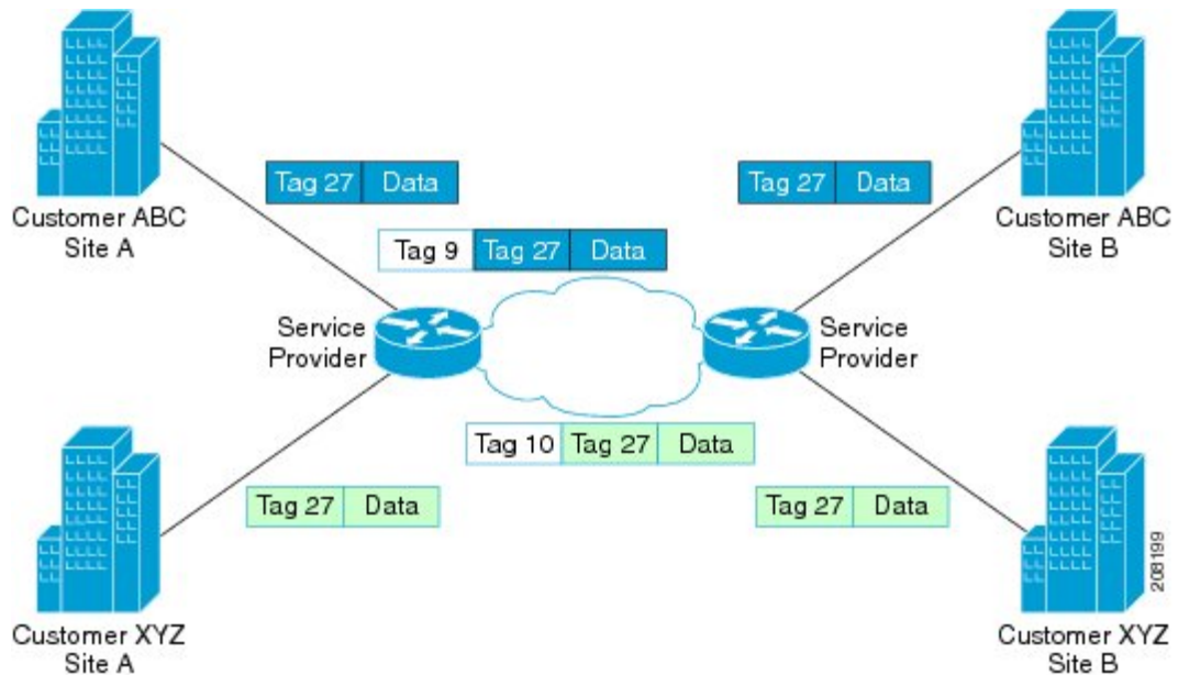
Figure 2: QinQ Tagging
