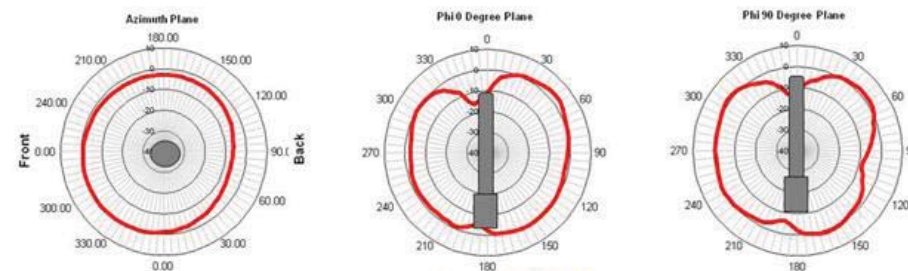
Frequency = 2700 MHz
