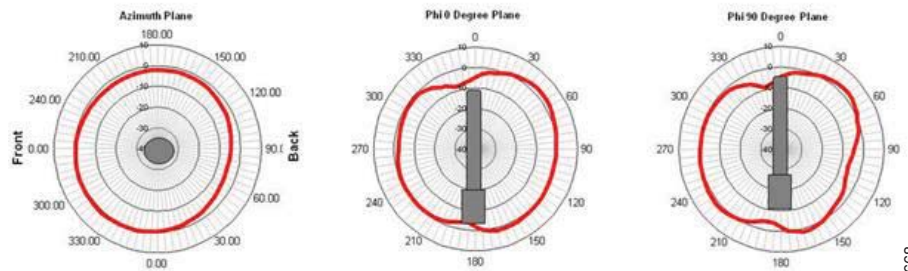
Frequency = 2500 MHz
