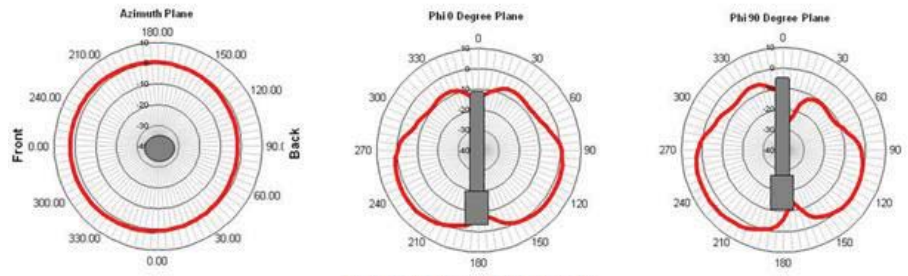
Frequency = 1710 MHz
