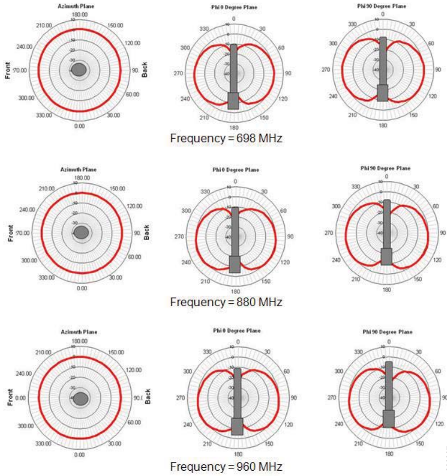
Figure 2 Outdoor Omnidirectional Antenna Radiation Patterns (1 of 2)
