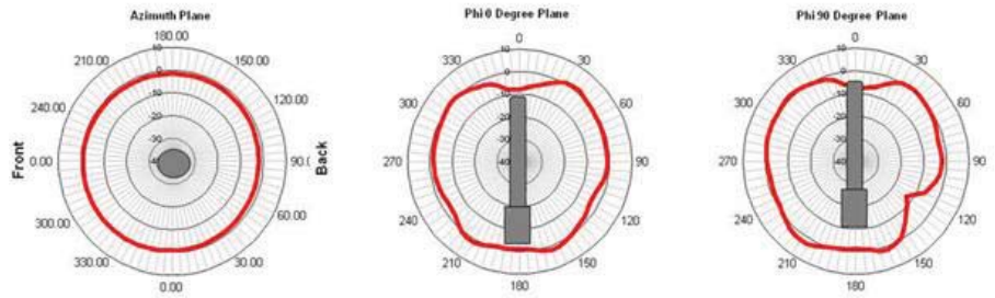
Frequency = 2170 MHz
