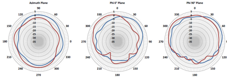
Figure 7: 1710 MHz Cellular Antenna Radiation Patterns
