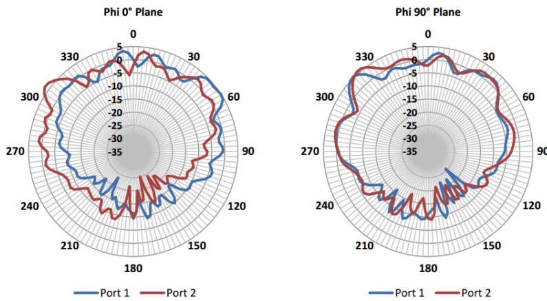
Figure 10: 5.9 GHz Antenna Radiation Patterns-Vertical Plane
