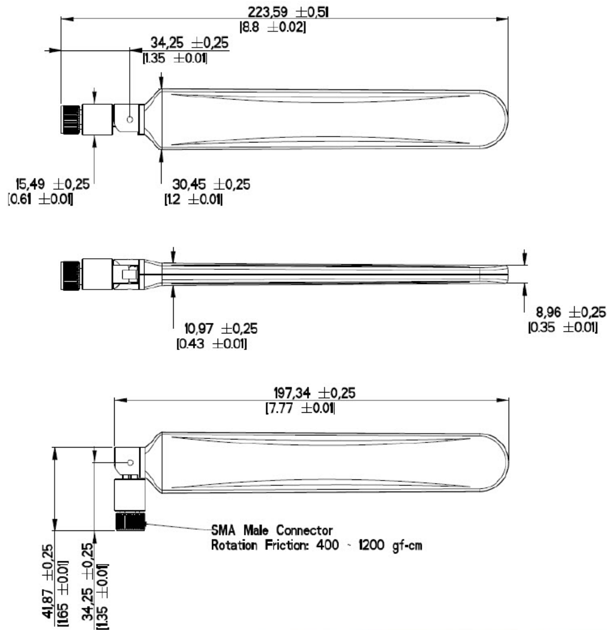
Figure 2: Mechanical Drawing
