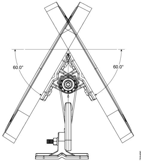
Figure 20: Elevation Adjustment
