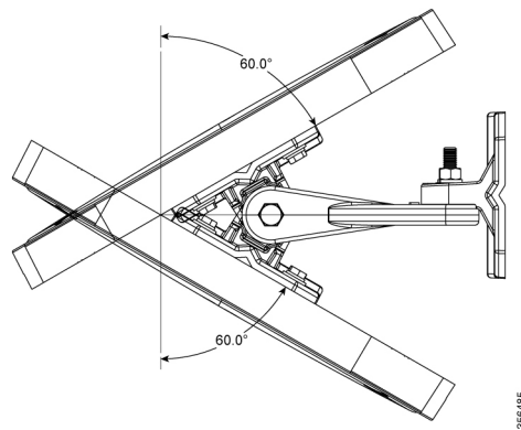
Figure 20: Elevation Adjustment
