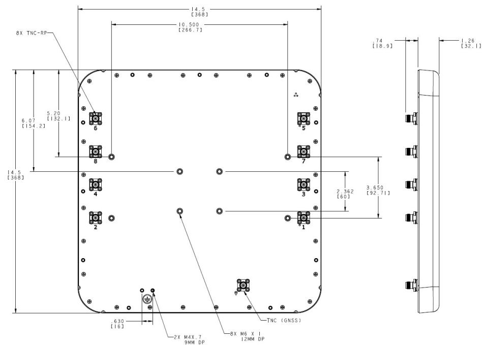
Figure 3: Antenna Dimensions
