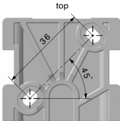
Figure 4: Anchor Holes
