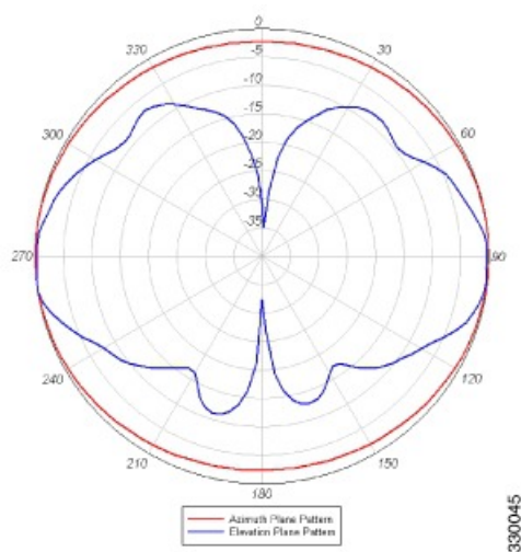
Figure 2: Azimuth and Elevation Plane Patterns for 5 GHz
