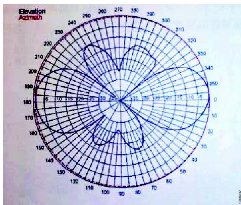
Figure 2: Outdoor Omnidirectional Antenna Radiation Pattern
