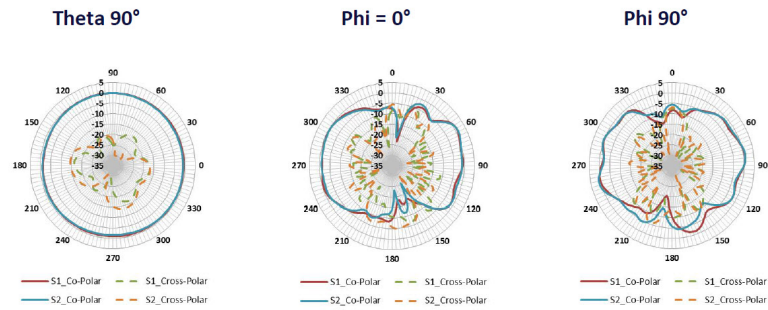
Figure 4: 863 MHz Radiation Pattern - With Ground Plane
