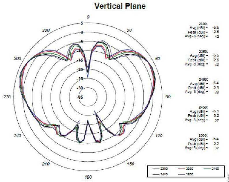
Figure 3: Radiation Pattern—Vertical Plane
