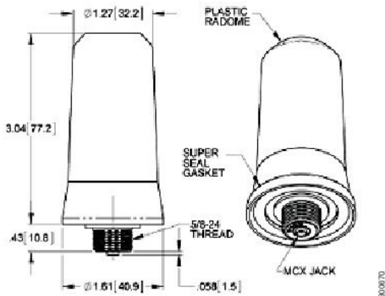
Figure 1: Monopole Antenna
