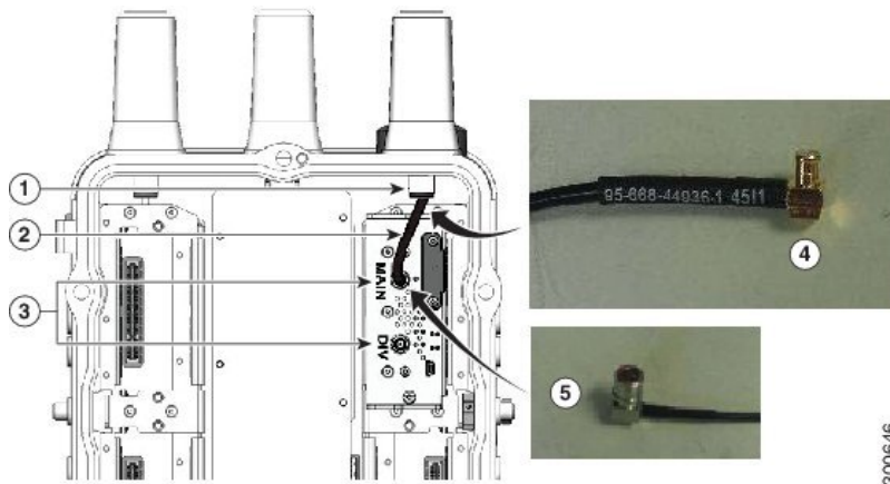
Figure 14: Antenna Details
