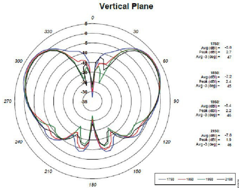
Figure 3: Radiation Pattern—Vertical Plane
