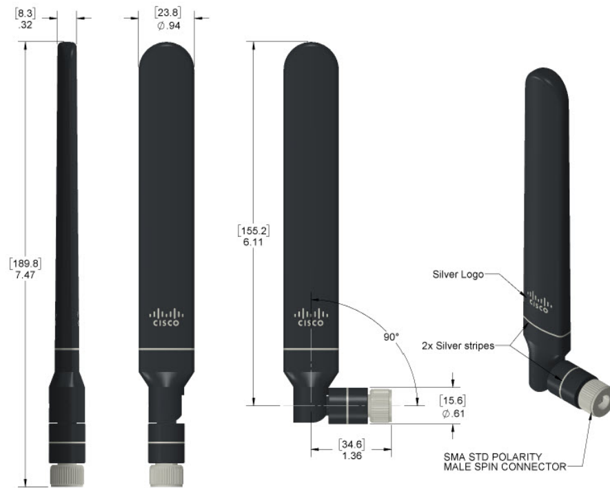
Figure 2: Mechanical Drawing
