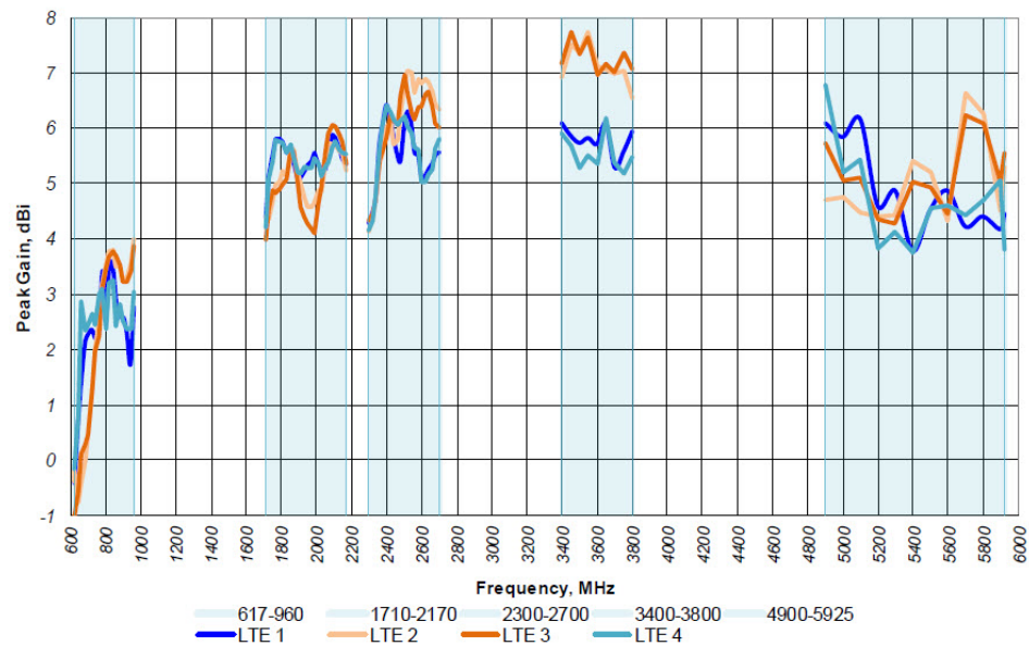
Figure 13: (LTE 1,2,3&amp;4) Measured with 2ft RG-316, Ø24in GP
