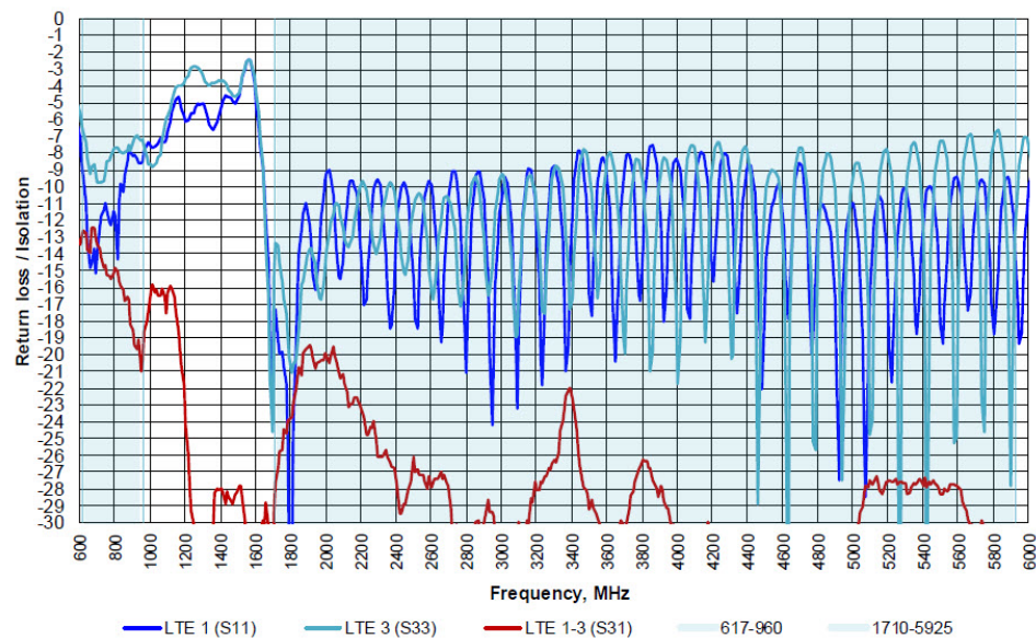
Figure 5: (LTE 1&amp;3) Measured with 2ft RG-316, Ø24in GP
