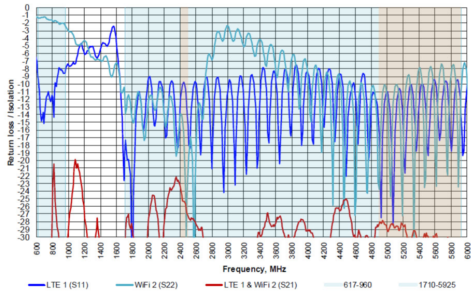
Figure 12: (LTE 1&amp; WiFi 2) Measured with 2ft RG-316, Ø24in GP
