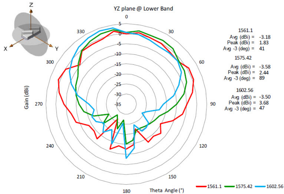
Figure 31: YZ plane @ Lower Band
