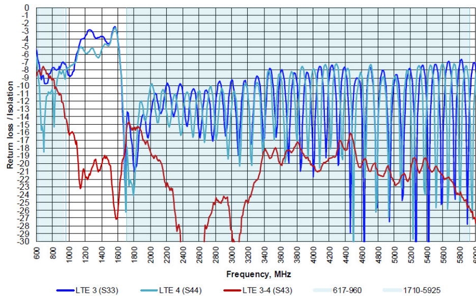
Figure 9: (LTE 3&amp;4) Measured with 2ft RG-316, Ø24in GP
