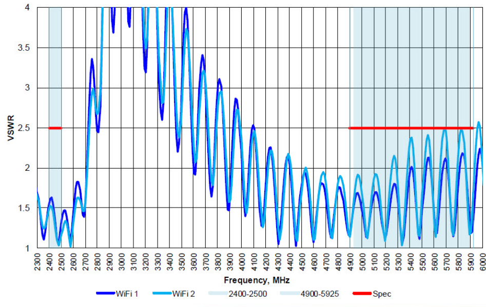
Figure 4: (WiFi 1&amp;2) Measured with 2ft RG-316, Ø24in GP
