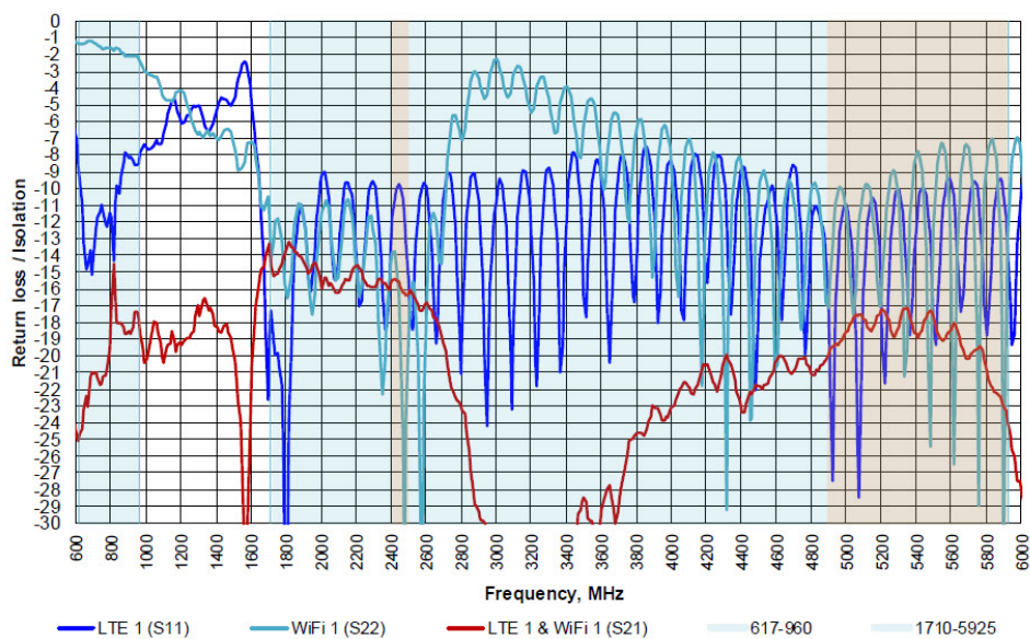
Figure 11: (LTE 1&amp; WiFi 1) Measured W/2ft RG-316, Ø24in GP
