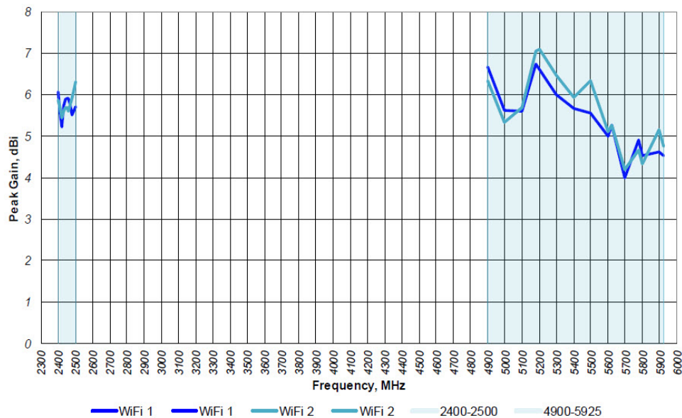
Figure 15: (WiFi 1&amp;2) Measured with 2ft RG-316, Ø24in GP
