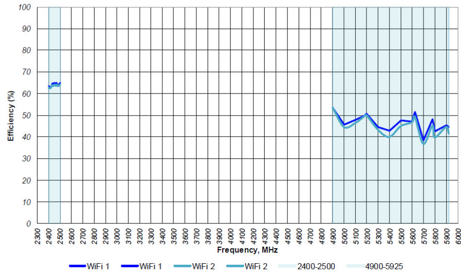
Figure 16: (WiFi 1&amp;2) Measured with 2ft RG-316, Ø24in GP
