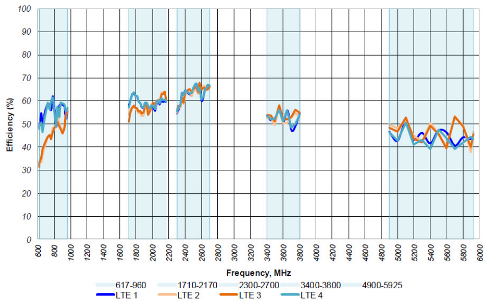
Figure 14: (LTE 1,2,3&amp;4) Measured with 2ft RG-316, Ø24in GP
