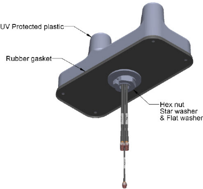
Figure 4: Mechanical Details 3
