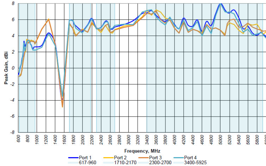
Figure 6: (LTE Ports 1-4) Measured W/2.3M (7.5ft) LMR-195 on Ø0.6M (2ft) GP
