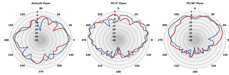
Figure 13: 5150 MHz WLAN Antenna Radiation Patterns
