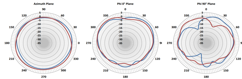
Figure 6: 1470 MHz Cellular Antenna Radiation Patterns
