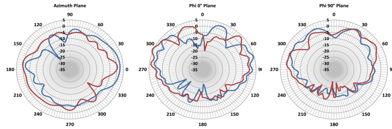
Figure 14: 5275 MHz WLAN Antenna Radiation Patterns
