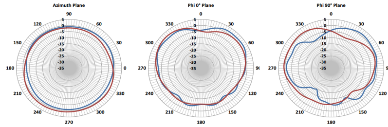
Figure 5: 960 MHz Cellular Antenna Radiation Patterns
