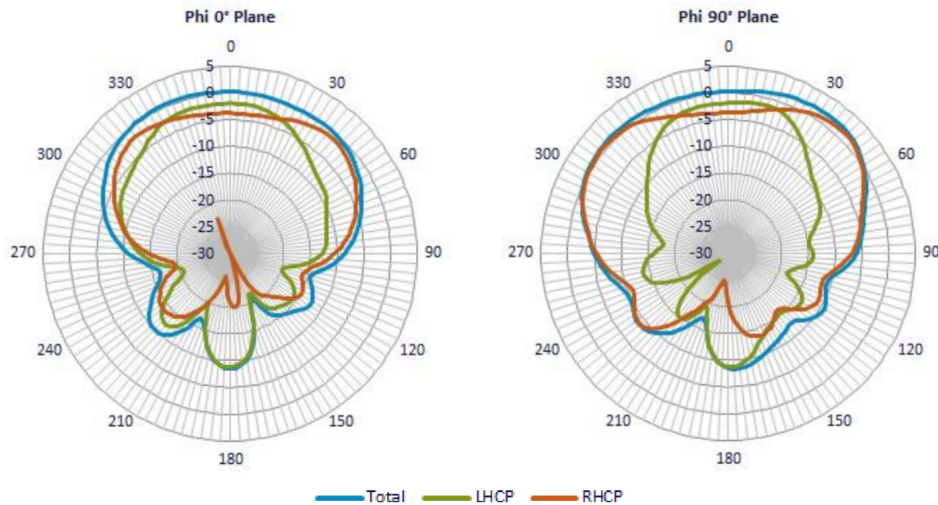
Figure 16: 1575 MHz GPS Antenna Radiation Patterns
