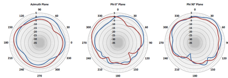
Figure 7: 1710 MHz Cellular Antenna Radiation Patterns
