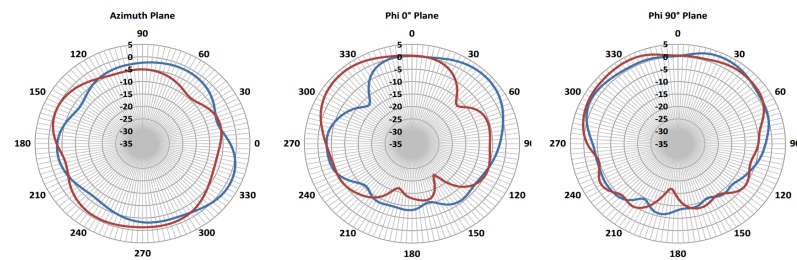
Figure 7: 1710 MHz Cellular Antenna Radiation Patterns
