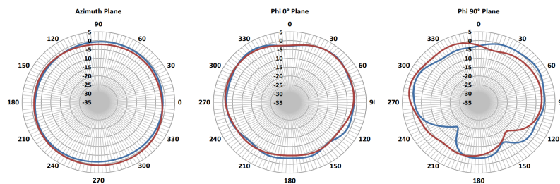
Figure 3: 698 MHz Cellular Antenna Radiation Patterns
