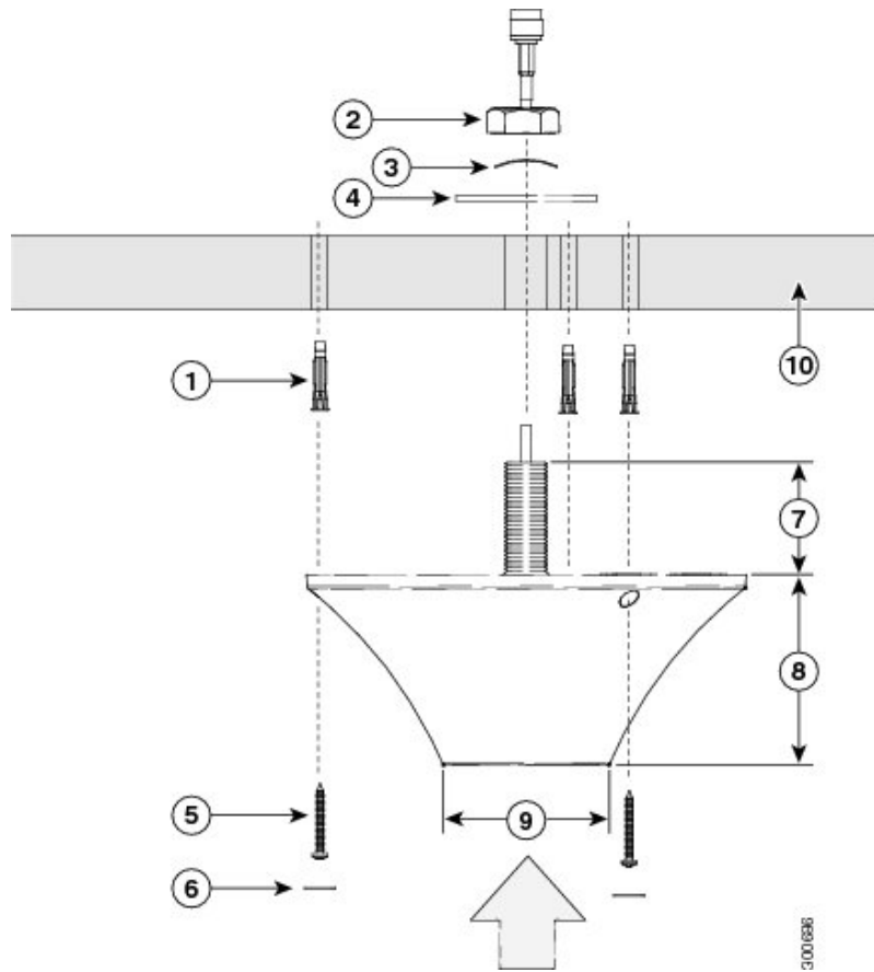
Figure 3: Antenna Details
