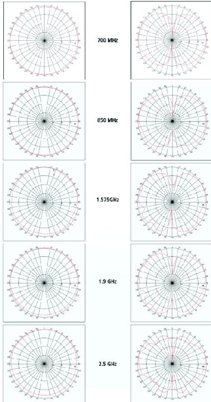
Figure 2: 4G Volcano Antenna Radiation Patterns
