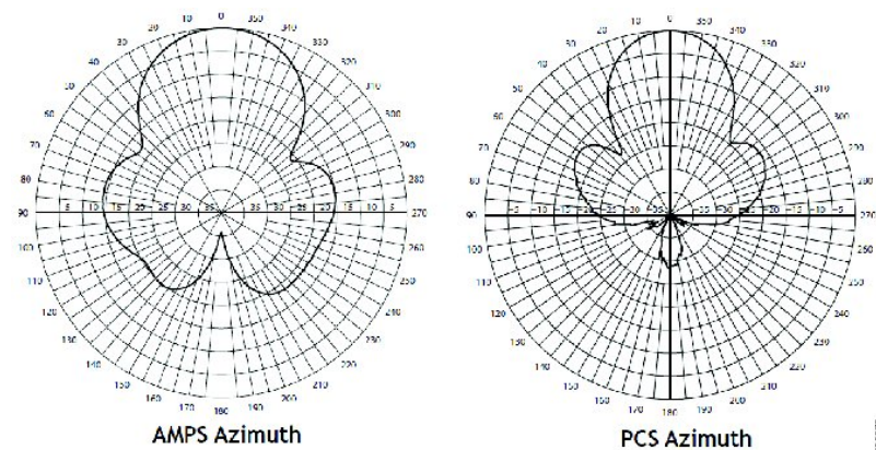
Figure 2: Outdoor 3G Antenna Radiation Patterns
