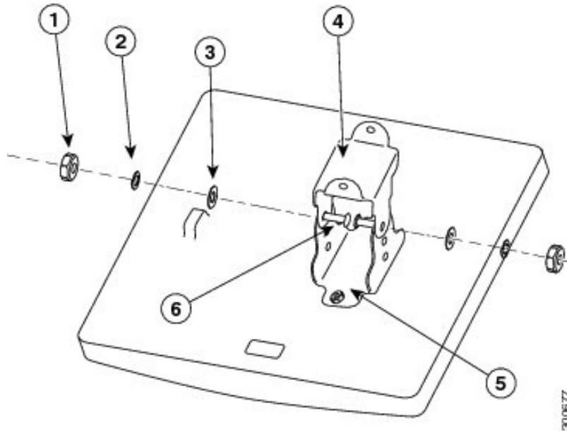
Figure 5: Elevation Brackets
