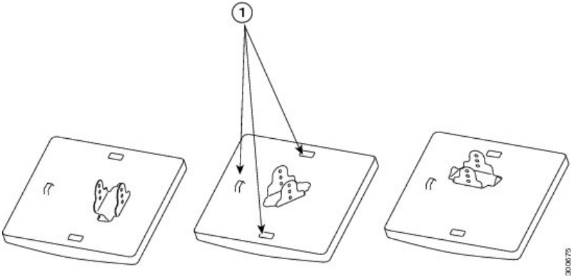
Figure 3: Antenna Polarization
