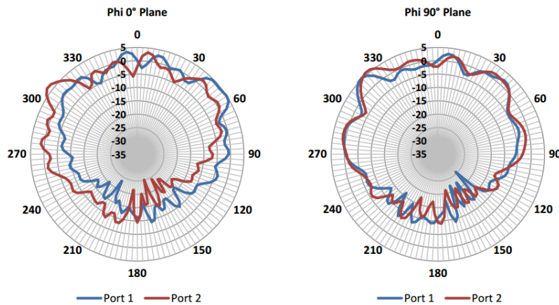
Figure 10: 5.9 GHz Antenna Radiation Patterns-Vertical Plane
