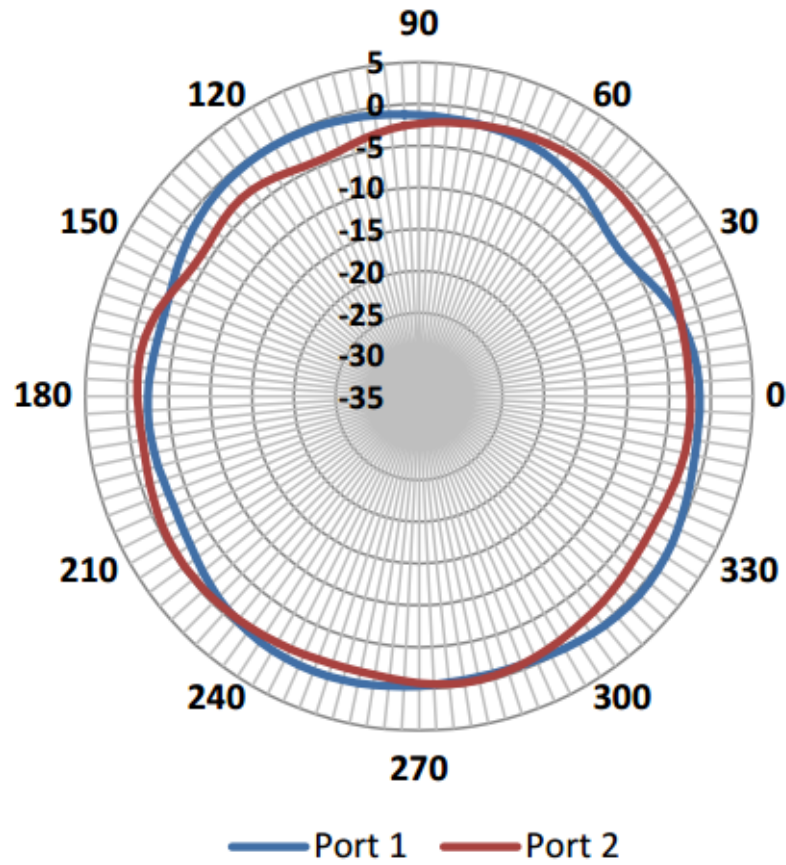
Figure 4: 2.46 GHz Antenna Radiation Patterns-Vertical Plane
