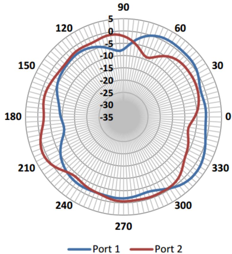
Figure 8: 5.55 GHz Antenna Radiation Patterns-Vertical Plane
