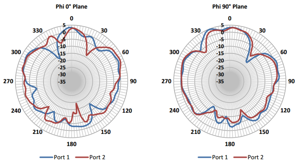
Figure 4: 2.46 GHz Antenna Radiation Patterns-Vertical Plane
