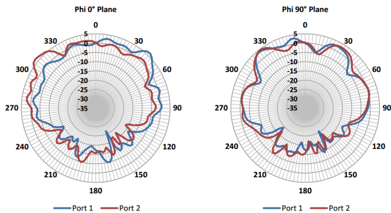
Figure 6: 4.9 GHz Antenna Radiation Patterns-Vertical Plane
