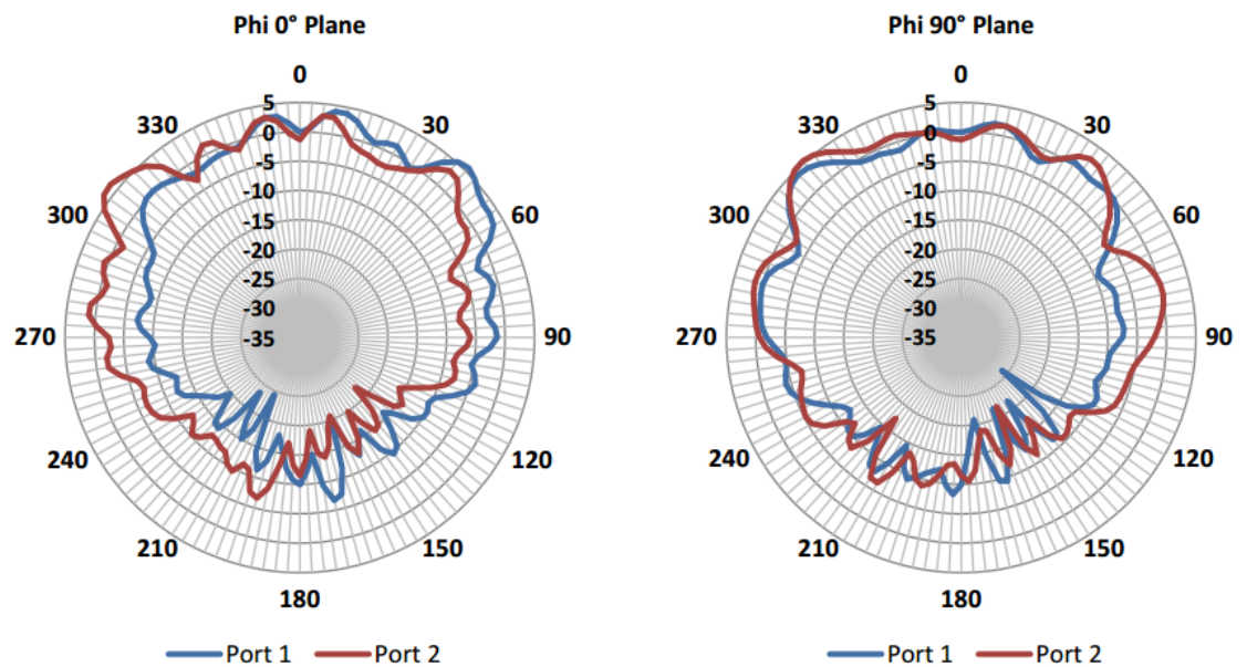
Figure 8: 5.55 GHz Antenna Radiation Patterns-Vertical Plane
