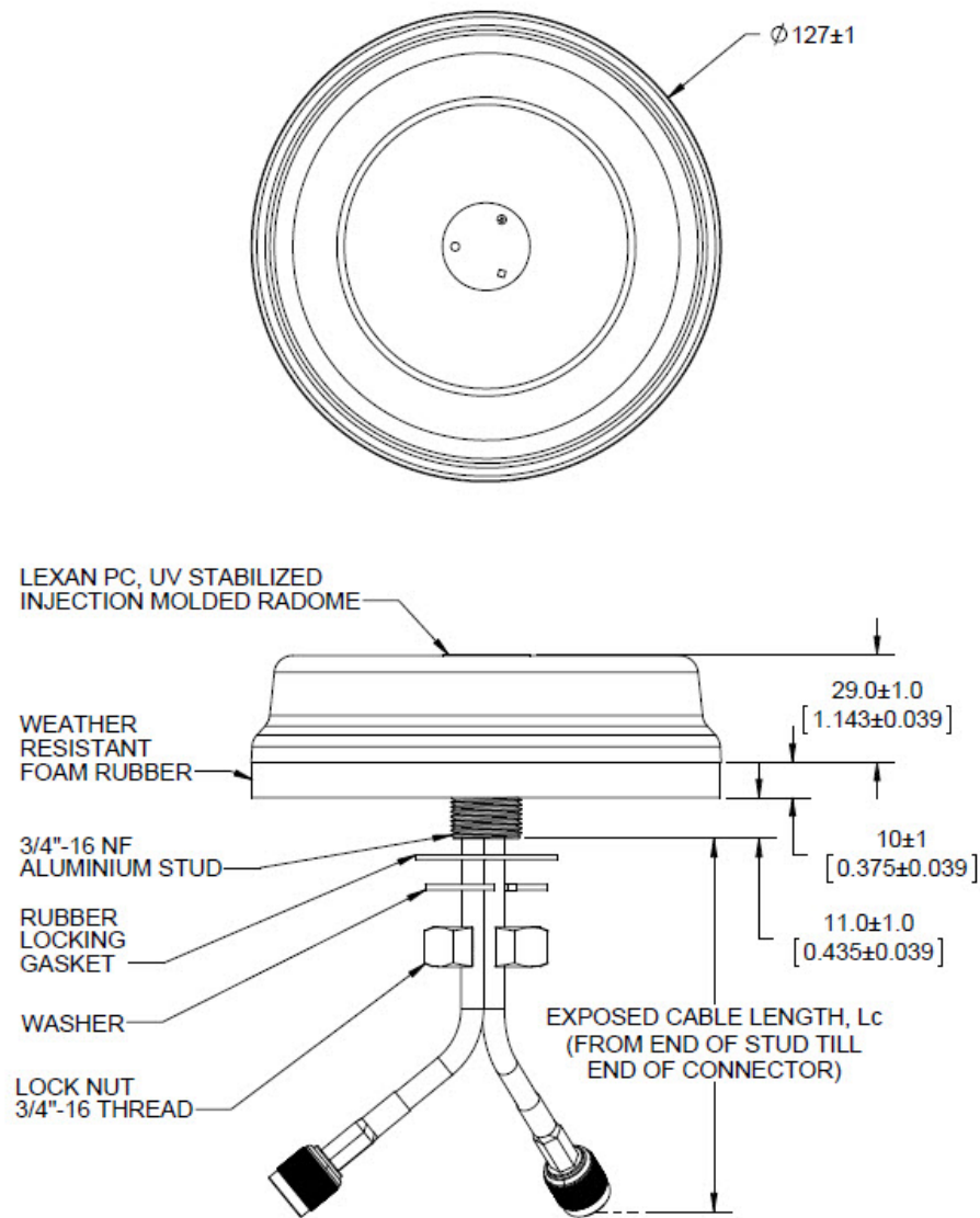
Figure 2: ANT-2-WLAN-D-0 Mechanical Details
