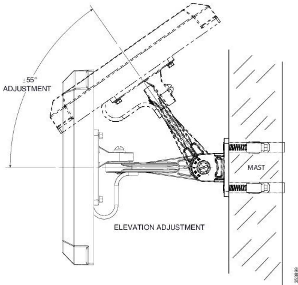
Figure 7: Elevation Adjustment
