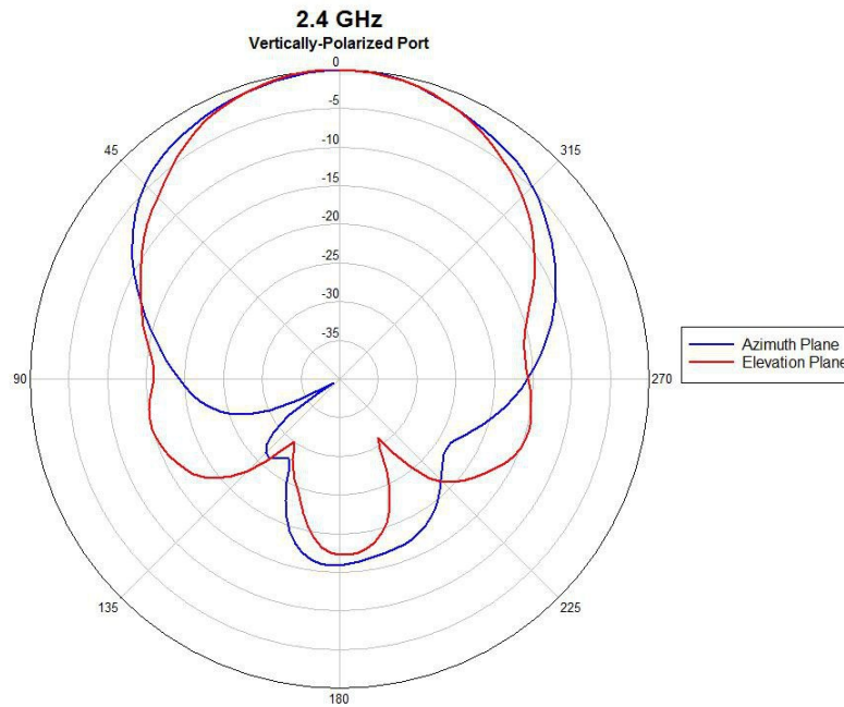
Figure 2: 2.4 GHz Vertical
