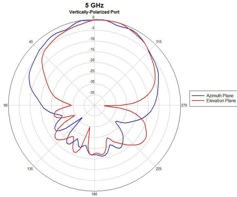
Figure 4: 5 GHz Vertical
