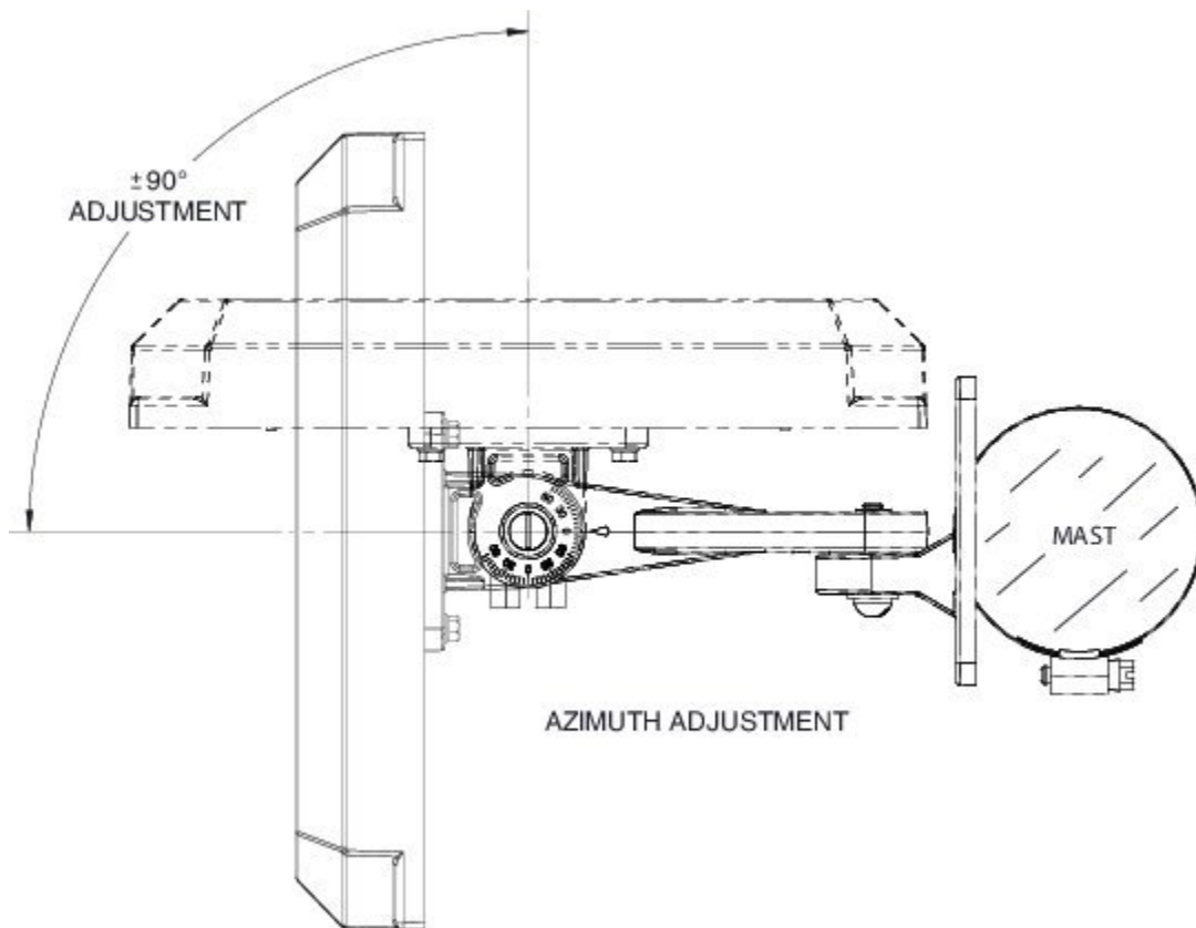
Figure 6: Azimuth Adjustment
