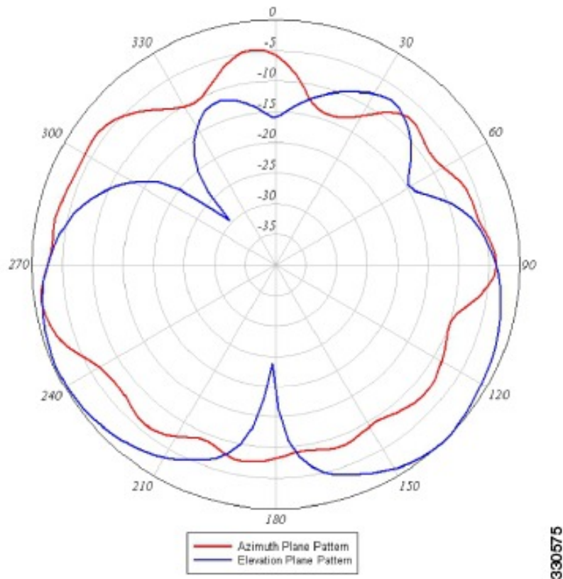
Figure 6: 5 GHz Element 3 Azimuth and Elevation Plane Patterns
