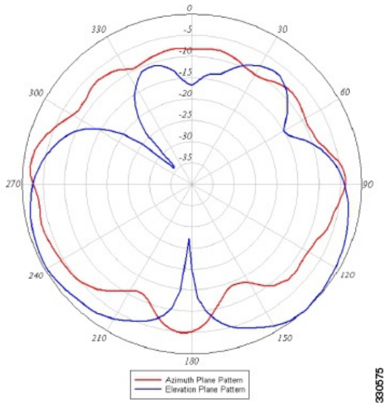
Figure 2: 5 GHz Element 1 Azimuth and Elevation Plane Patterns
