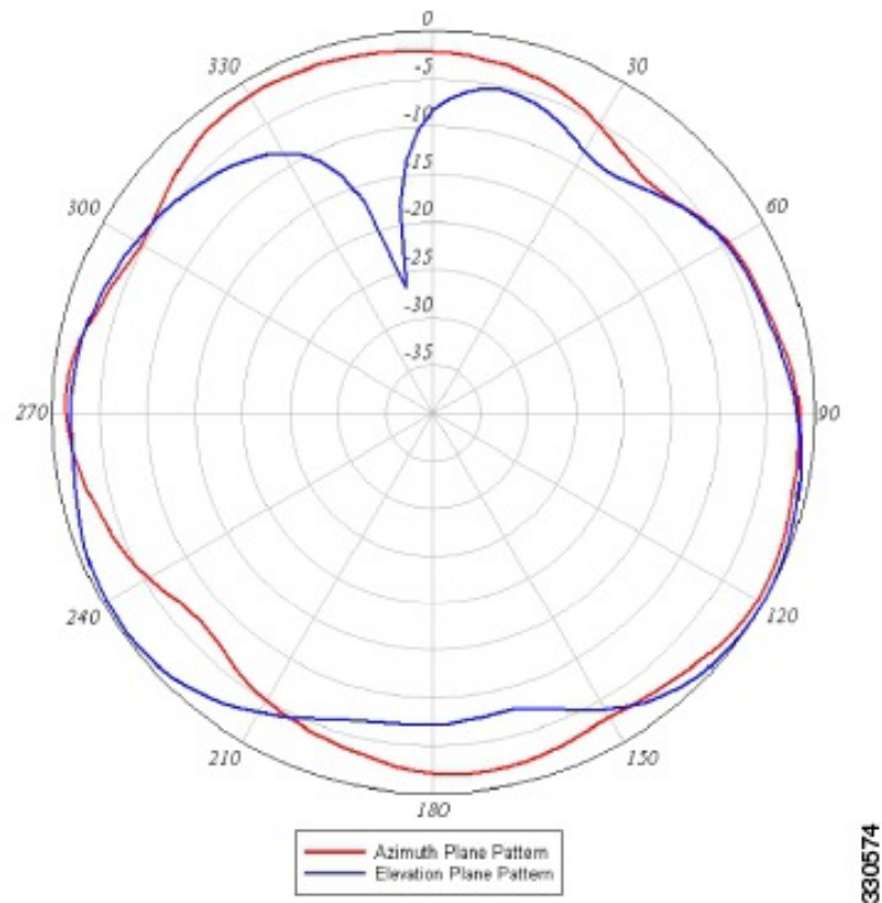
Figure 3: 2.4 GHz Element 2 Azimuth and Elevation Plane Patterns
