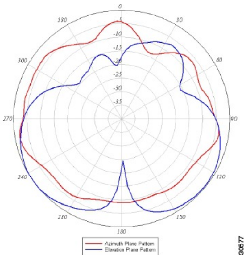
Figure 8: 5 GHz Element 4 Azimuth and Elevation Plane Patterns
