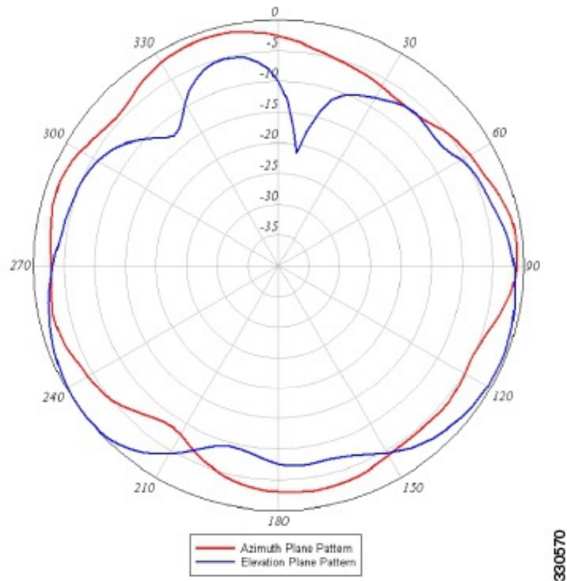
Figure 7: 2.4 GHz Element 4 Azimuth and Elevation Plane Patterns
