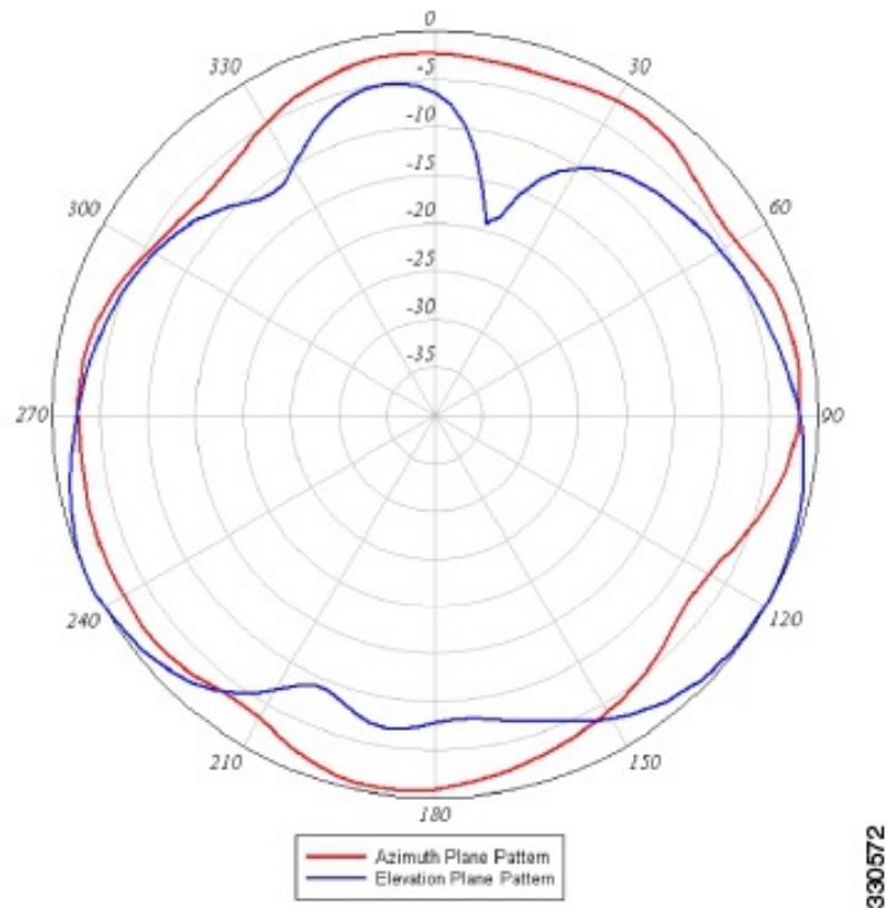
Figure 5: 2.4 GHz Element 3 Azimuth and Elevation Plane Patterns
