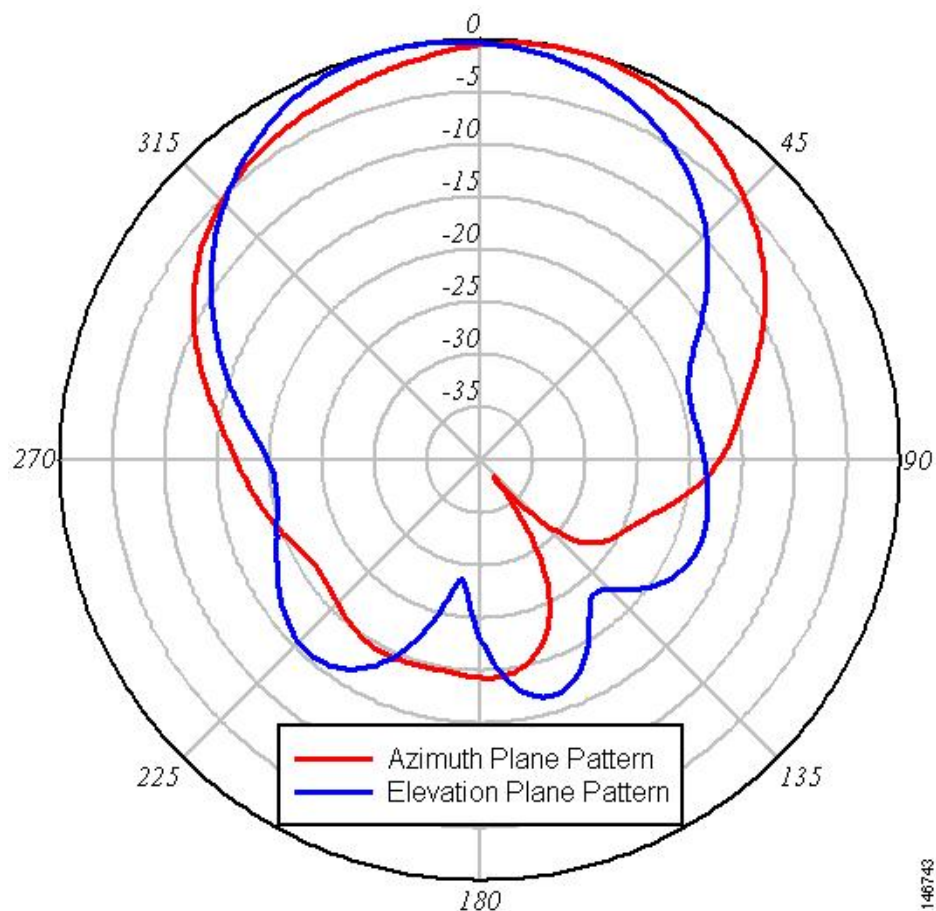
Figure 1: Left Antenna Azimuth and Elevation Pattern
