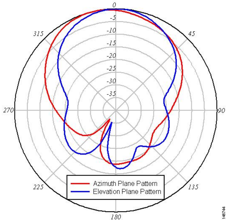
Figure 2: Right Antenna Azimuth and Elevation Pattern
