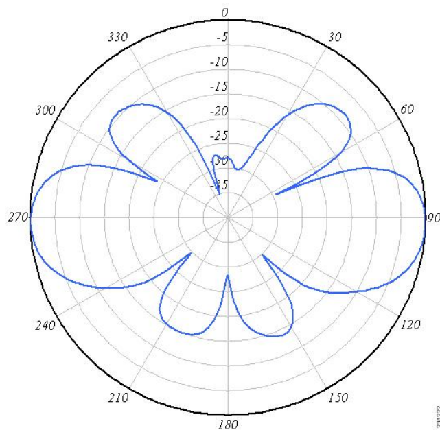
Figure 2: Elevation Radiation Pattern
