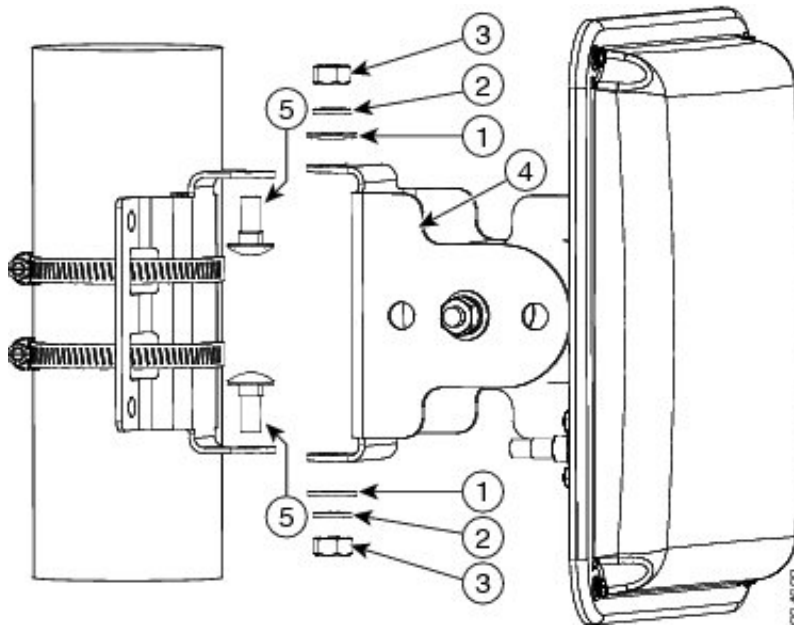
Figure 5: Attaching Antenna Assembly
