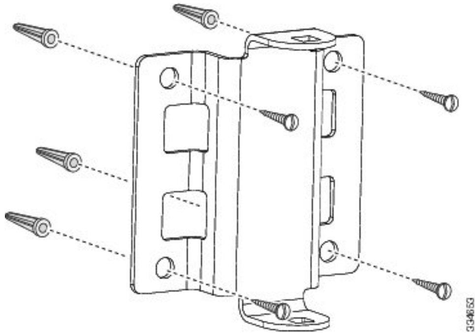
Figure 9: Wall Mounting
