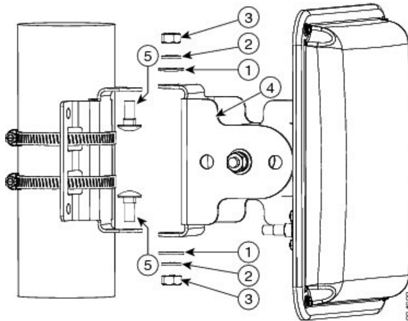
Figure 11: Attaching Antenna Assembly
