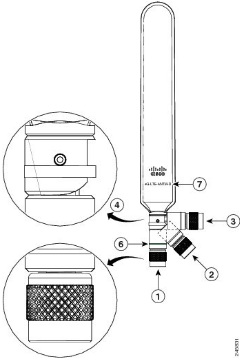
Figure 1: Cisco 4G-LTE-ANTM-D Ominidirectional Dipole Antenna, TNC Connector, and Articulation Joint
