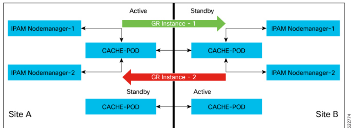
Figure 34: IPAM Architecture
