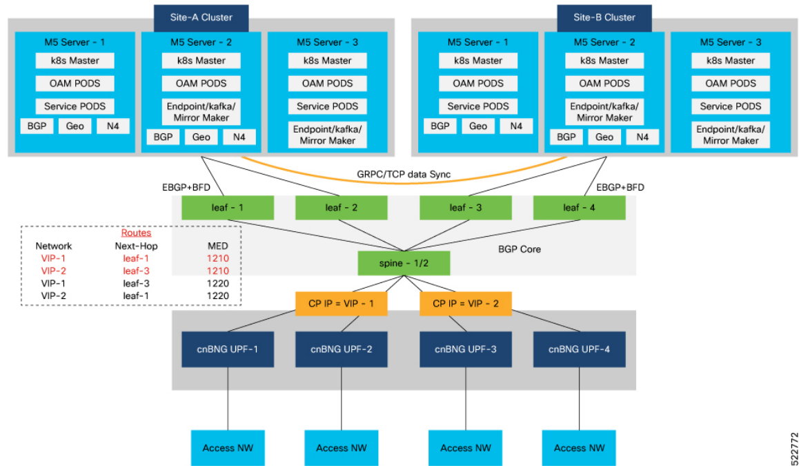
Figure 29: cnBNG CP Geo Redundancy Architecture
