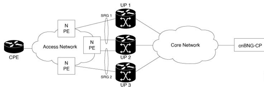
Figure 28: Subscriber Redundancy Group
