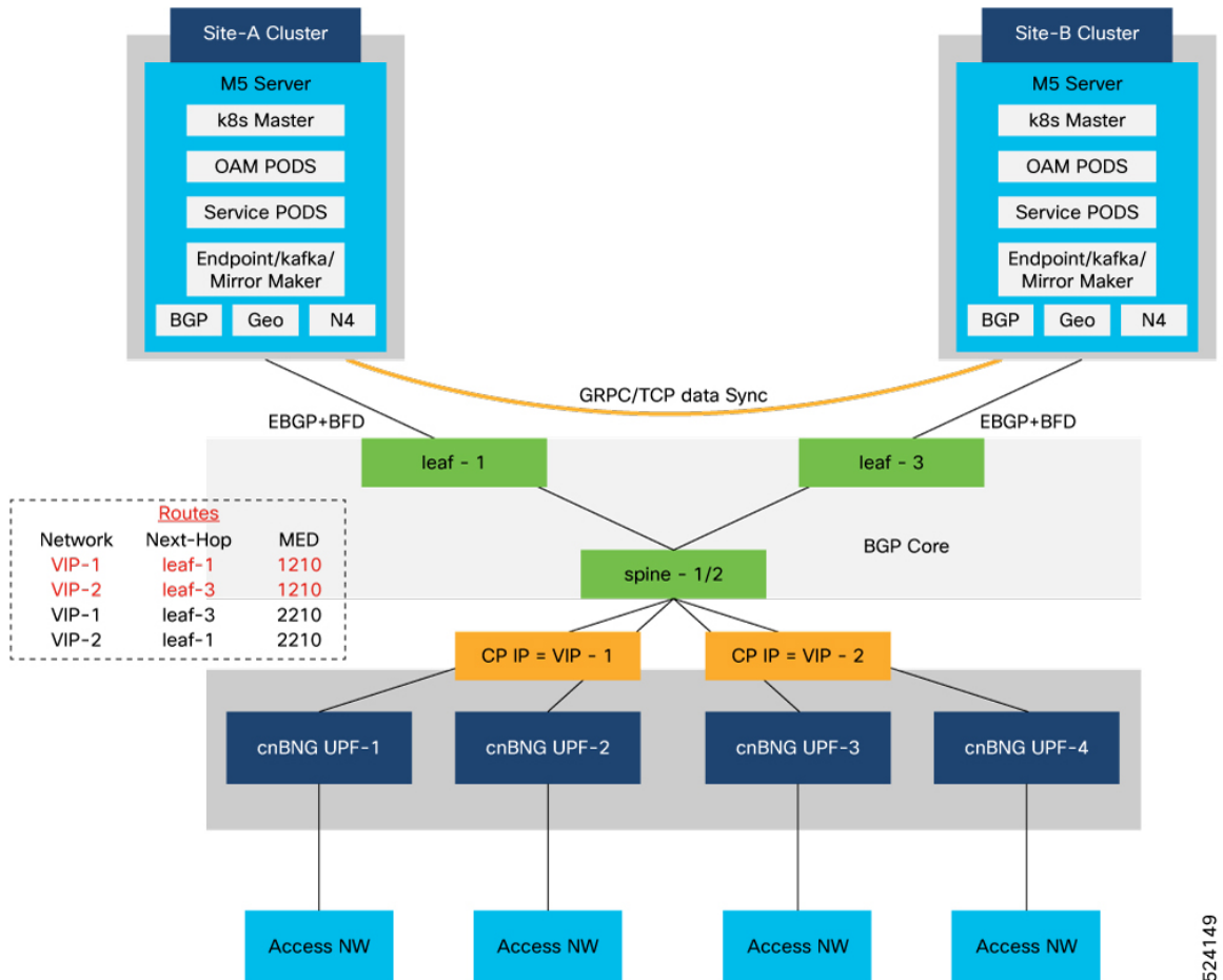
Figure 24: AIO CP Geo Redundancy Architecture
