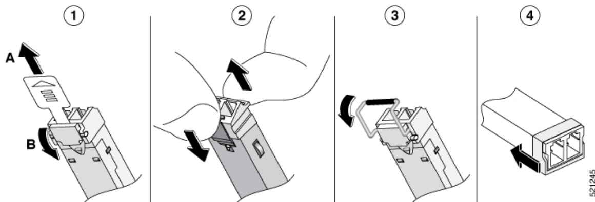
Figure 23: Disconnecting SFP Latch Mechanisms
