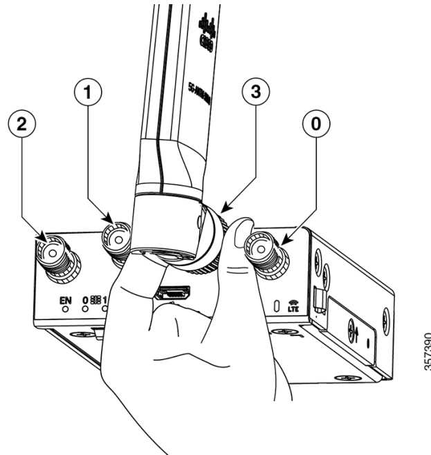
Figure 4: Attaching the Antennas
