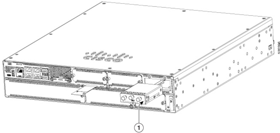
Figure 2: Pluggable Interface Module in a Cisco 8300-2N2S-4T2X|6T
