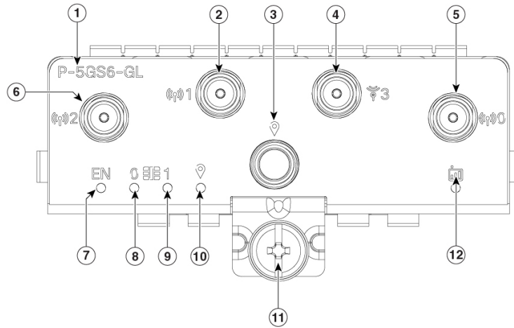
Figure 3: 5G Pluggable Interface Module - P-5GS6-GL
