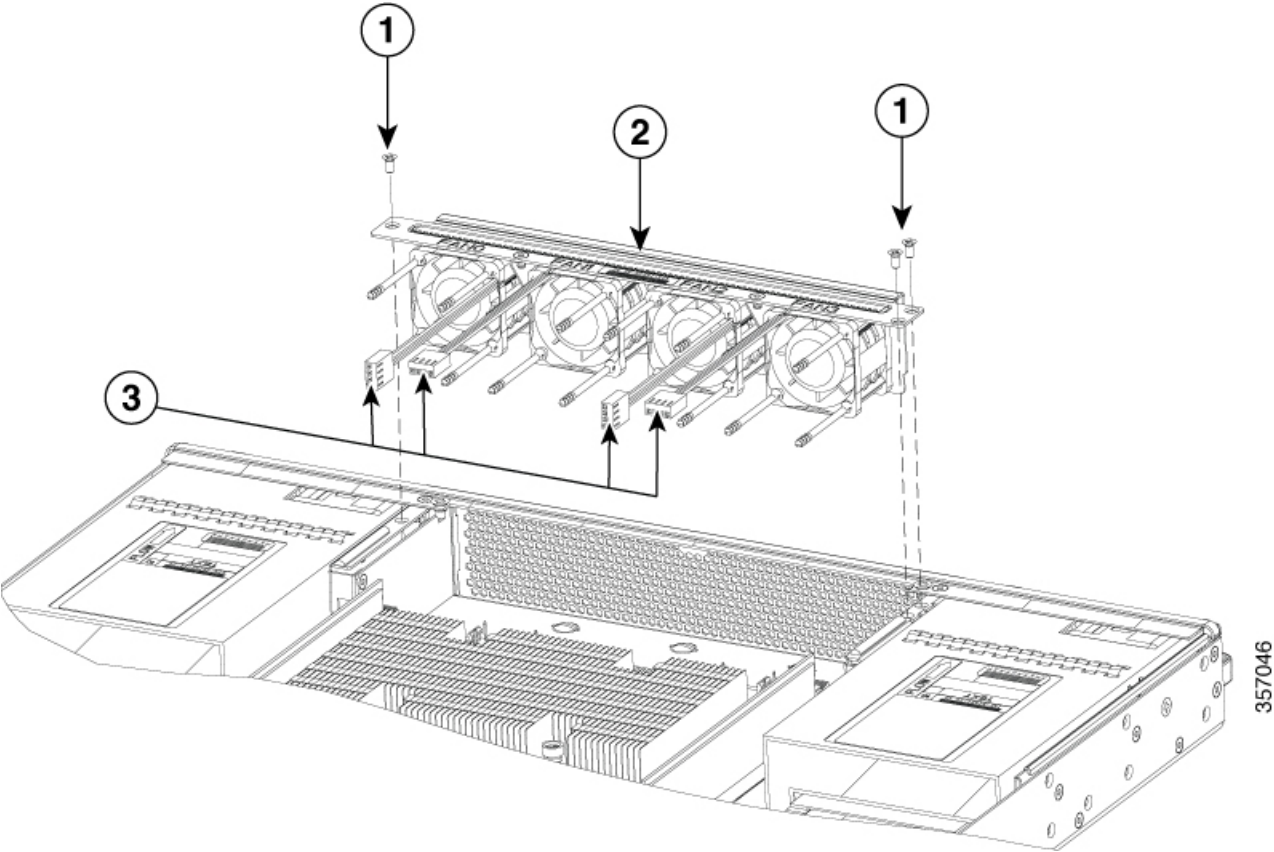
Figure 19: Fan tray
