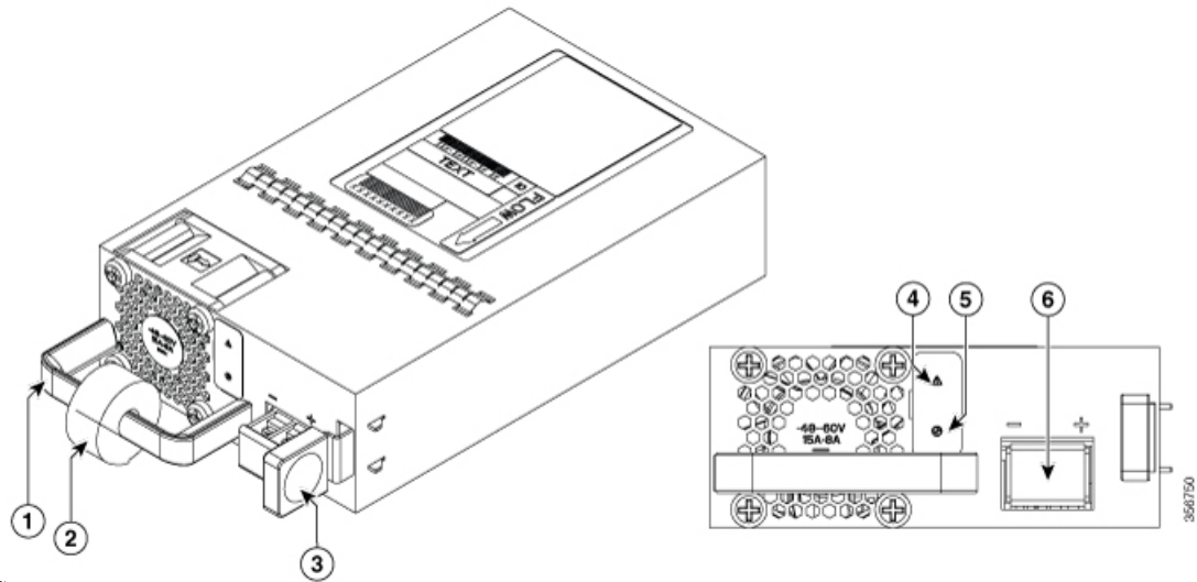
Figure 12: DC power
