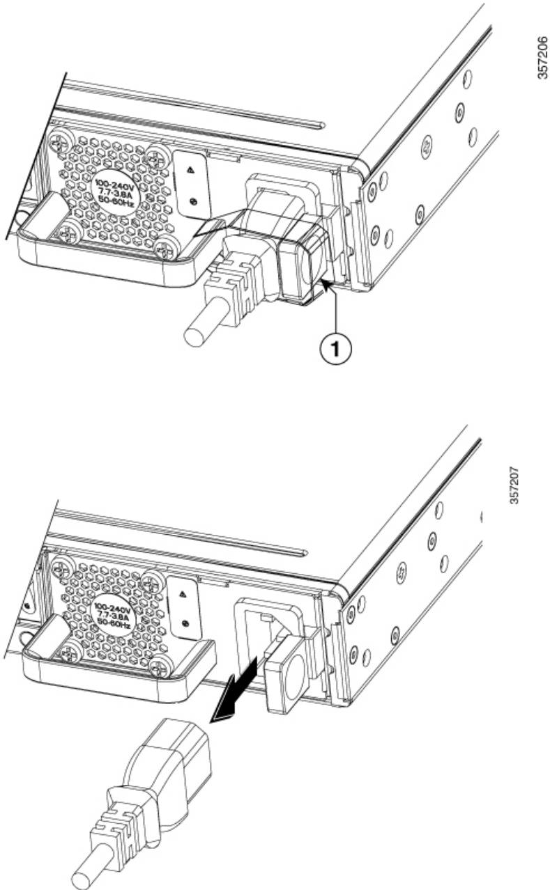
Figure 8: Replace the AC power supply
