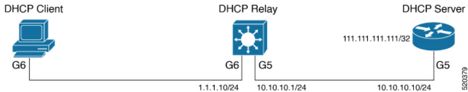
Figure 3: Topology Showing DHCP Client with GigabitEthernet Interface
