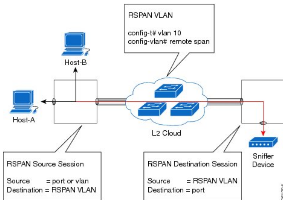
Figure 1: RSPAN Traffic
