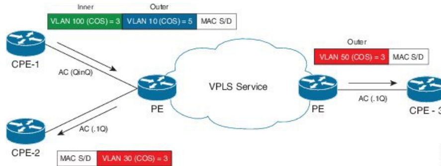
Figure 2: 2:1 VLAN Translation
