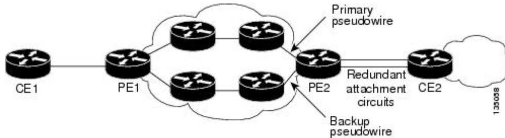
Figure 3: Pseudowire Redundancy
