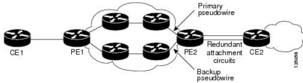
Figure 3: Pseudowire Redundancy
