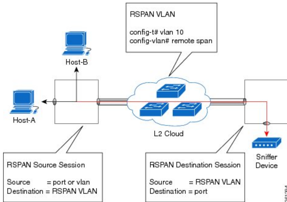
Figure 2: RSPAN Traffic
