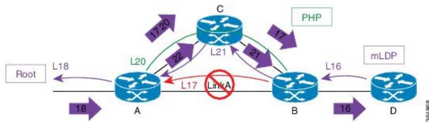
Figure 13: Re-optimization - Make-Before-Break
