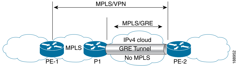
Figure 9 P-to-PE Tunneling
