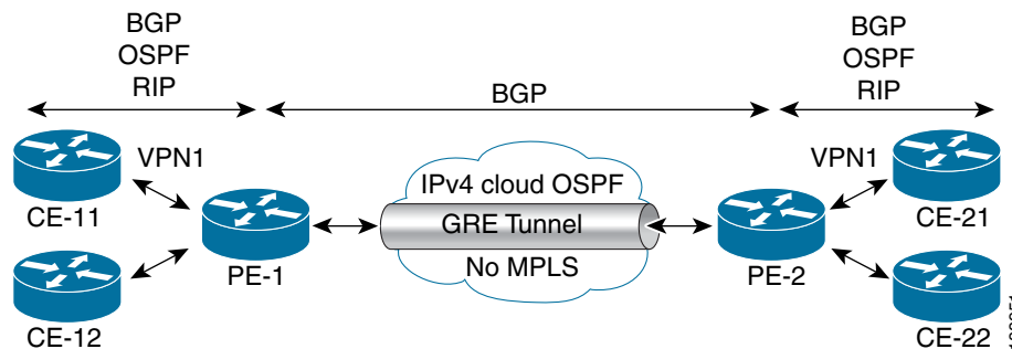
Figure 8 PE-to-PE Tunneling
