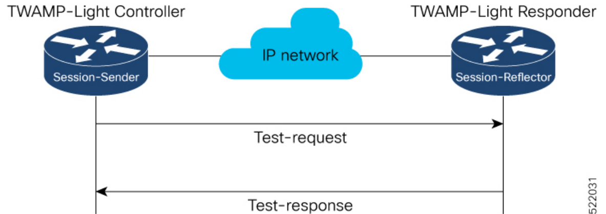
Figure 8: TWAMP-Light test-session
