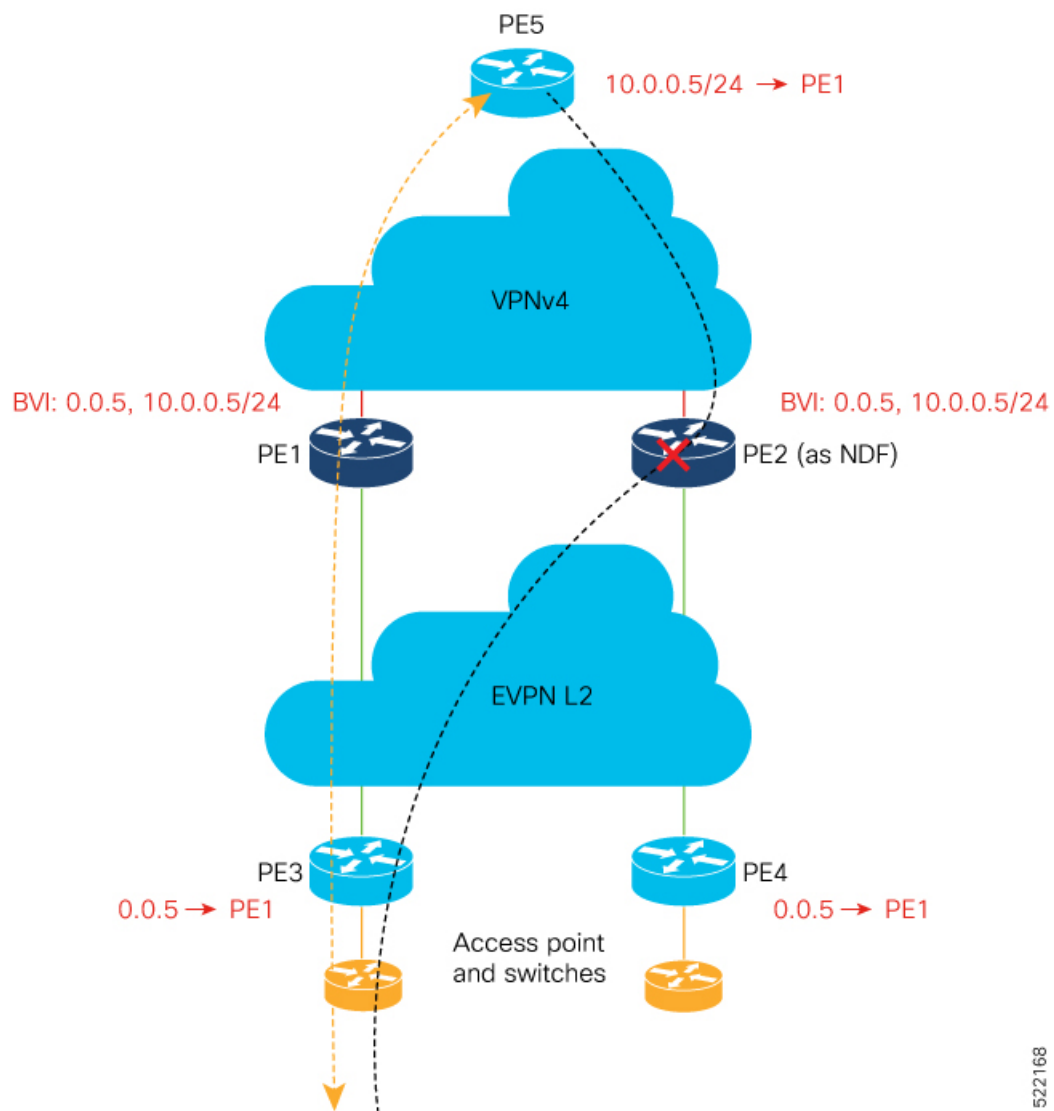
Figure 3: Topology
