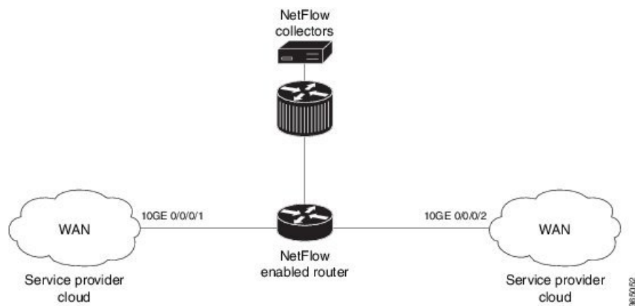
Figure 1: SP-PE Topology
