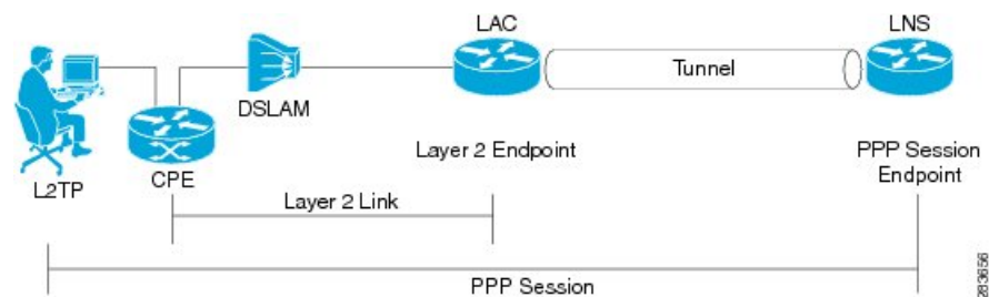
Figure 3: LAC Session
