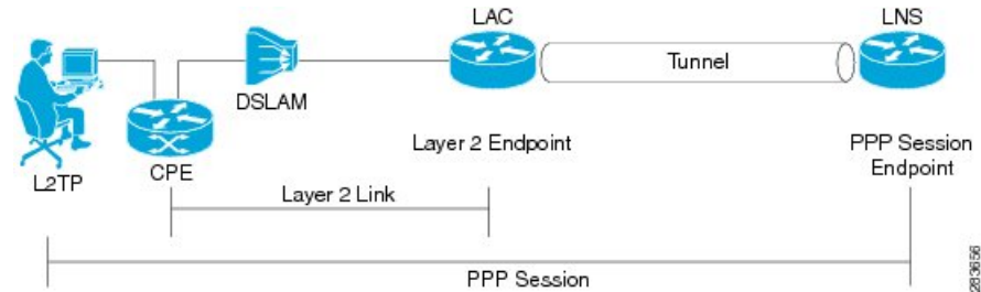
Figure 8: LAC Session
