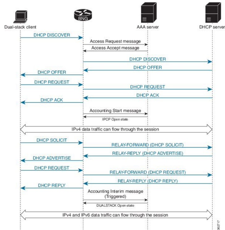
Figure 48: Call Flow of IPoE Dual-Stack - IPv4 Address-Family Starts First
