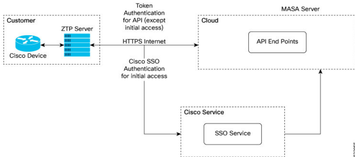
Figure 20: Components of the Authentication Flow
