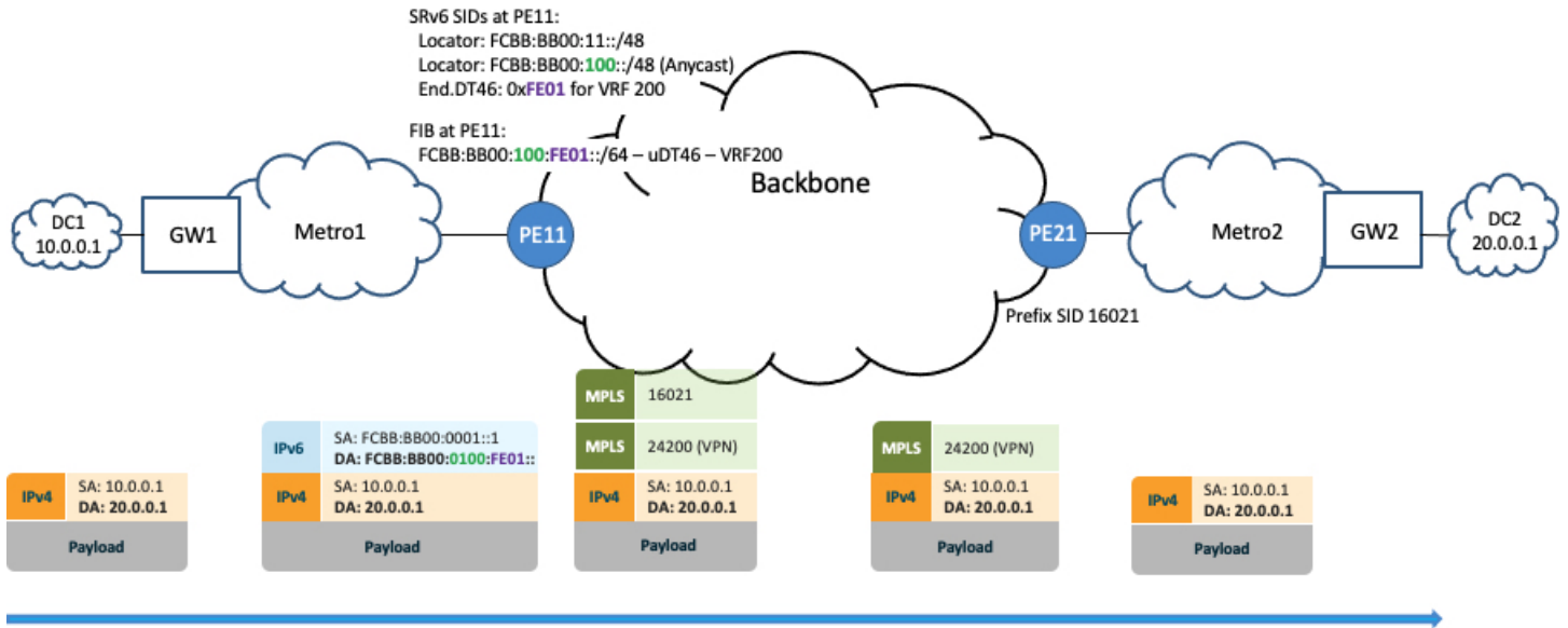
Figure 14: Best Effort Traffic (Traffic Direction – DC1 to DC2)
