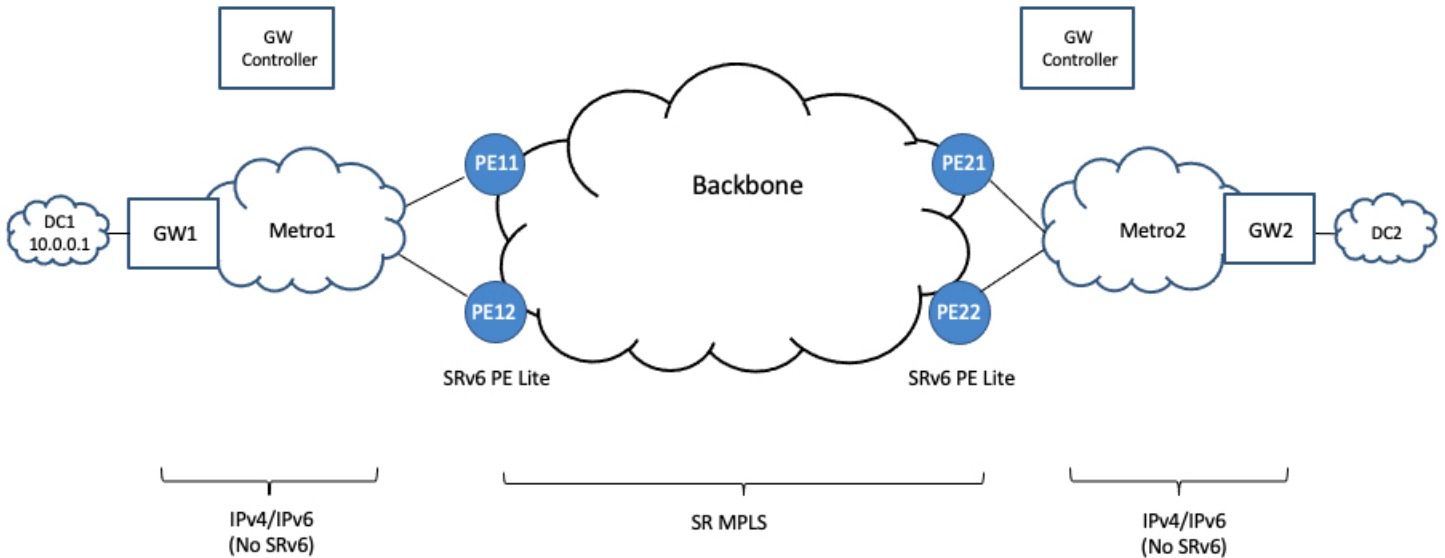
Figure 10: Example Topology
