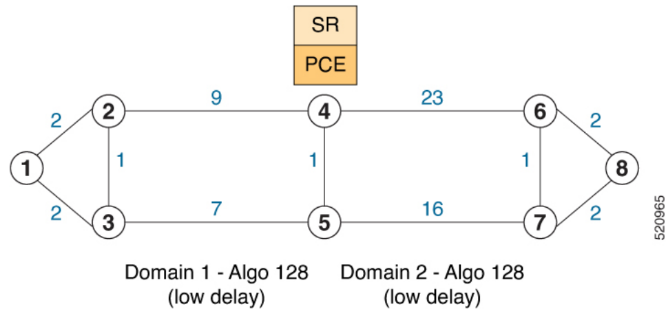
Figure 31: Multi-Domain Topology
