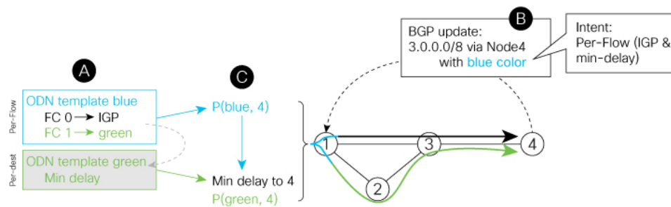
Figure 22: PFP with ODN Example
