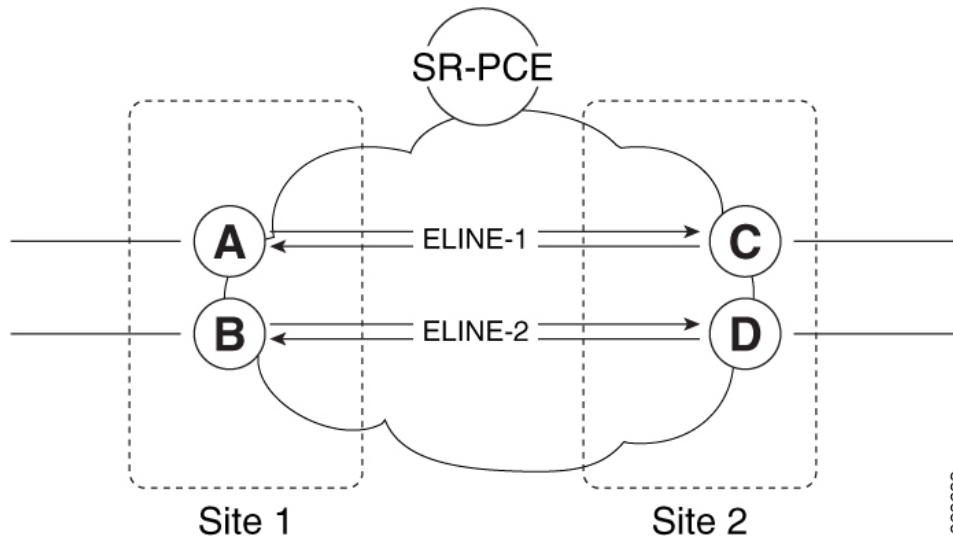
Figure 19: Topology for Use Case: SR-ODN for EVPN-VPWS
