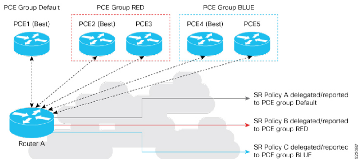
Figure 20: Example: PCE Groups
