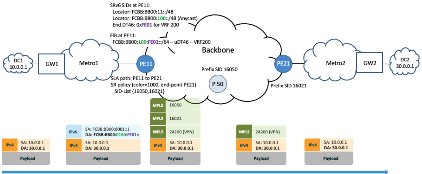
Figure 15: SLA Traffic (Traffic Direction – DC1 to DC2)
