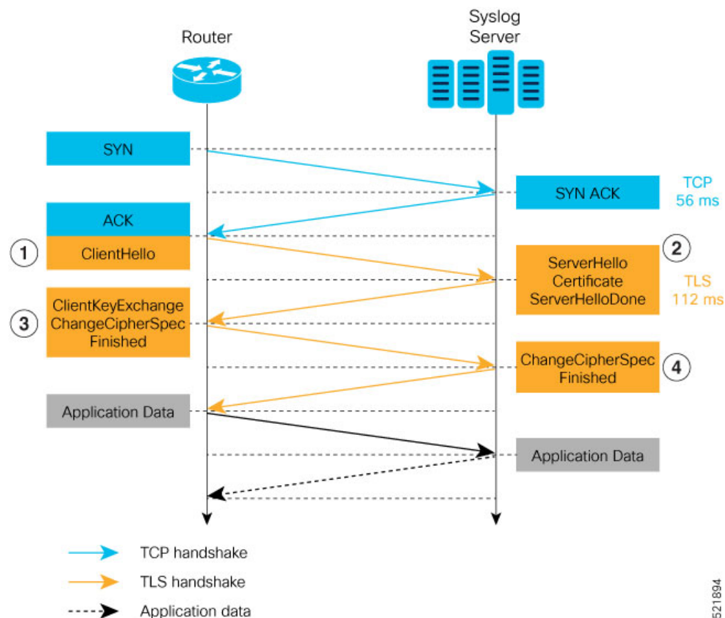
Figure 1: TLS Handshake
