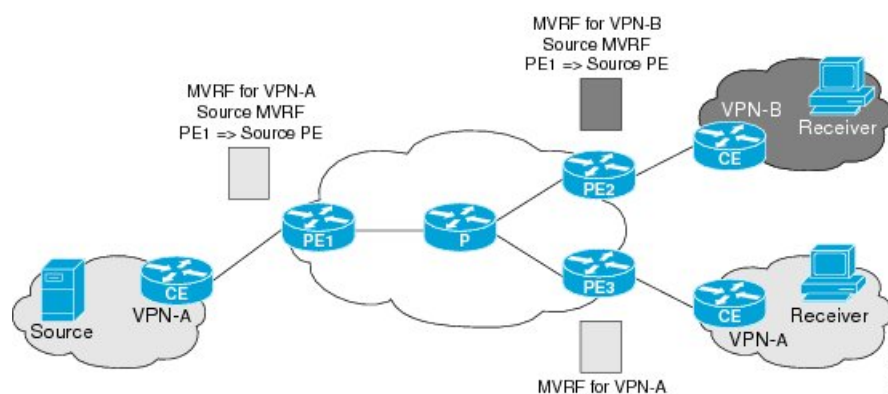
Figure 8: Components of an Extranet MVPN
